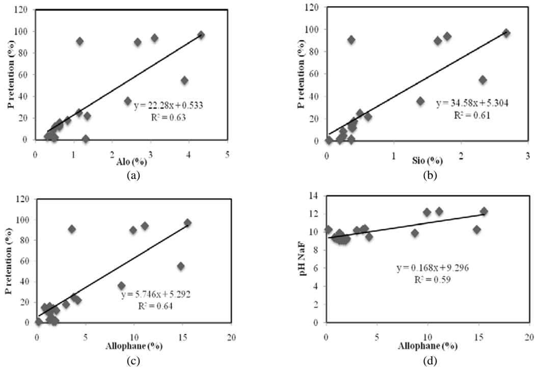
Figure 2. Correlation between various soil properties : (a) Relationship between Al_o vs P-retention, (b) Si_o vs P-retention, (c) Allophane vs P-retention, (d) Allophane vs pH-NaF of the volcanic ash soils from North Sulawesi
