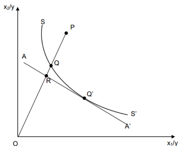
Figure 2. Technical efficiency, allocative efficiency, and economic efficiency
